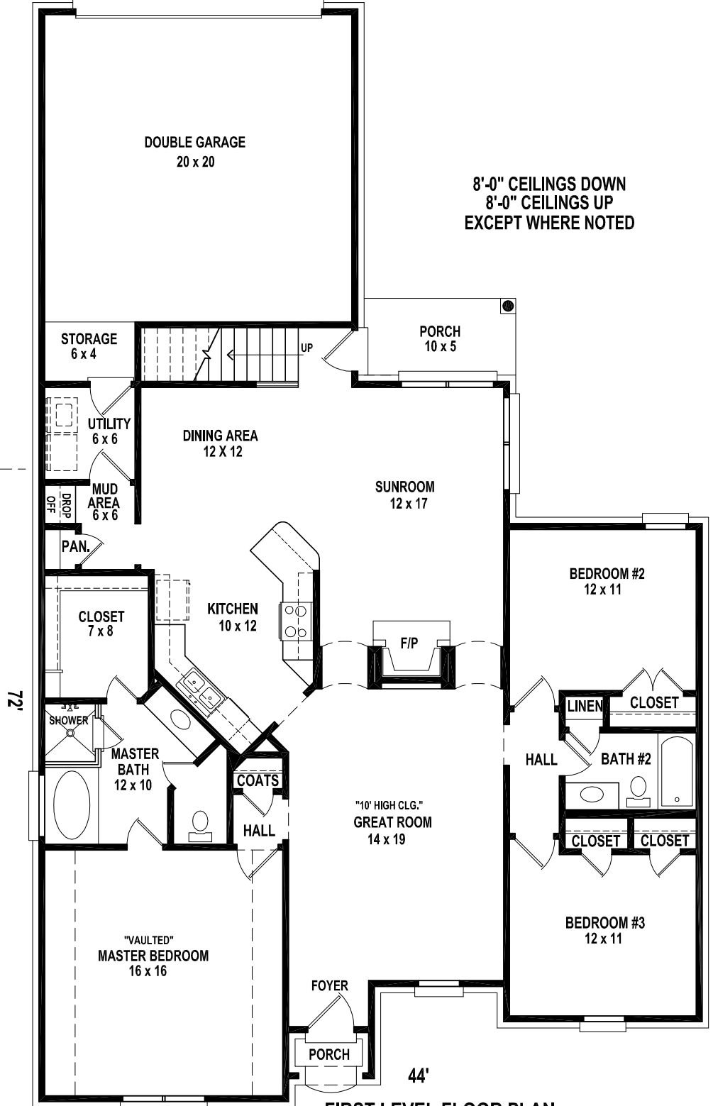
FIRST LEVEL FLOOR PLAN
