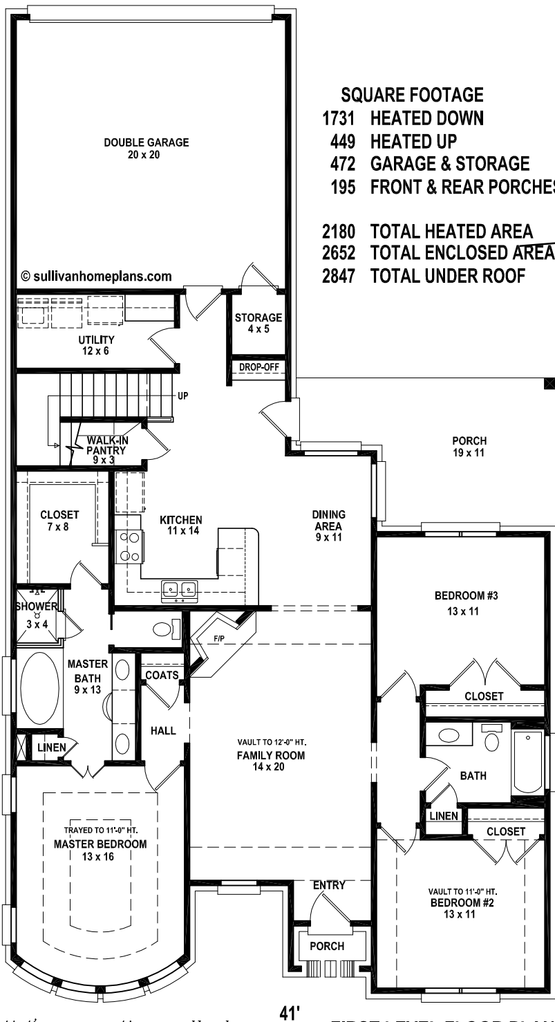
FIRST LEVEL FLOOR PLAN
